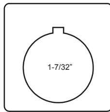
LEGD013 2-1/2 x 2
