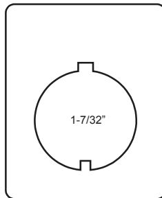
LEGD013 2-1/2 x 2
